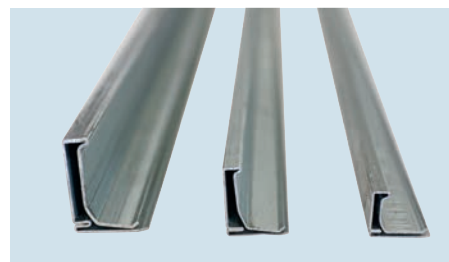
Luftkanal-Profile 40, 30, 20 mm / Airduct profiles 40,30,20 mm
