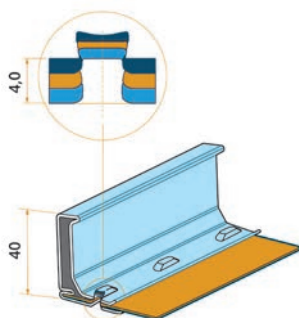
Luftkanal-Schnitt 3-lagig / 3-layer airduct cross-section
